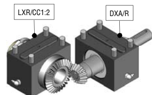
Support DXA/R with shaft Combined with Support LXR/CC1:2
