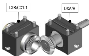
Support DXA/R with shaft Combined with Support LXR/CC1:1
